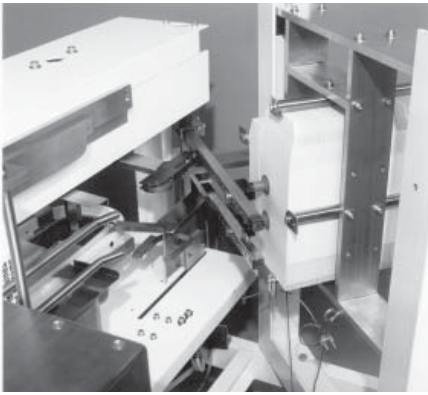
Carton pulled from magazine via vacuum.
