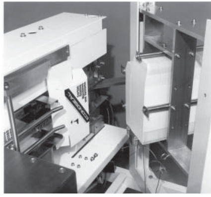
Carton automatically erected.
