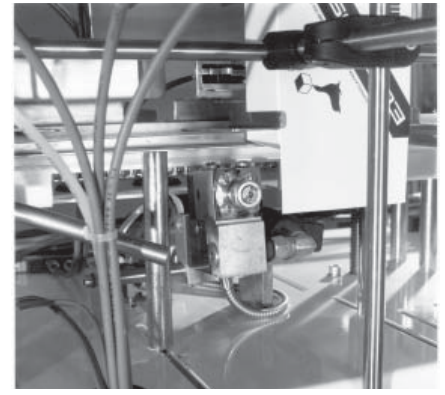
Bottom of carton is closed - either glue (as shown) or tuck method.
