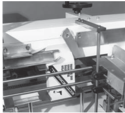
Top dust flaps of carton are closed.
