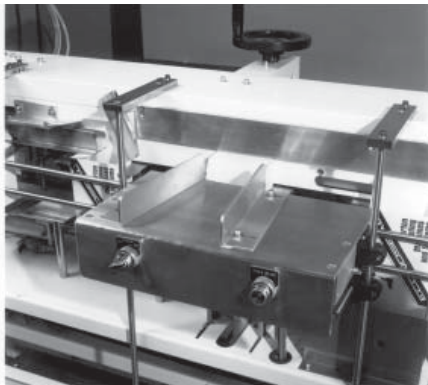
Bottom closed carton is presented at single load station.
